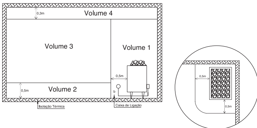
ABNT NBR5410 – Volumes da Sauna
